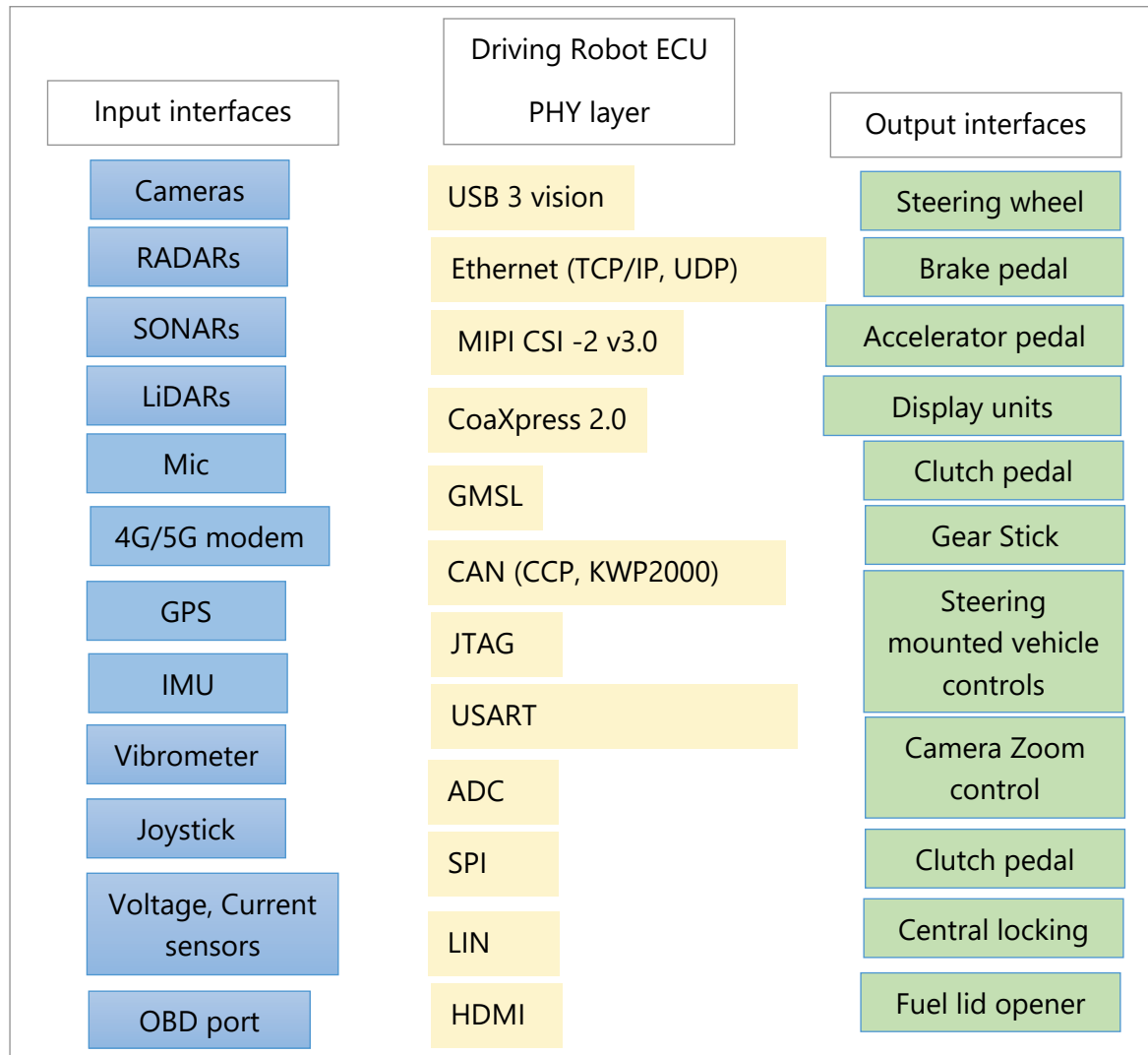
Figure 9: Connection network interfaces within the vehicle
