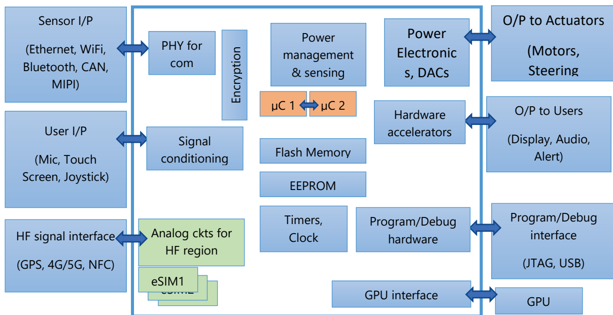
Figure 5: Block diagram of the ECU hardware
