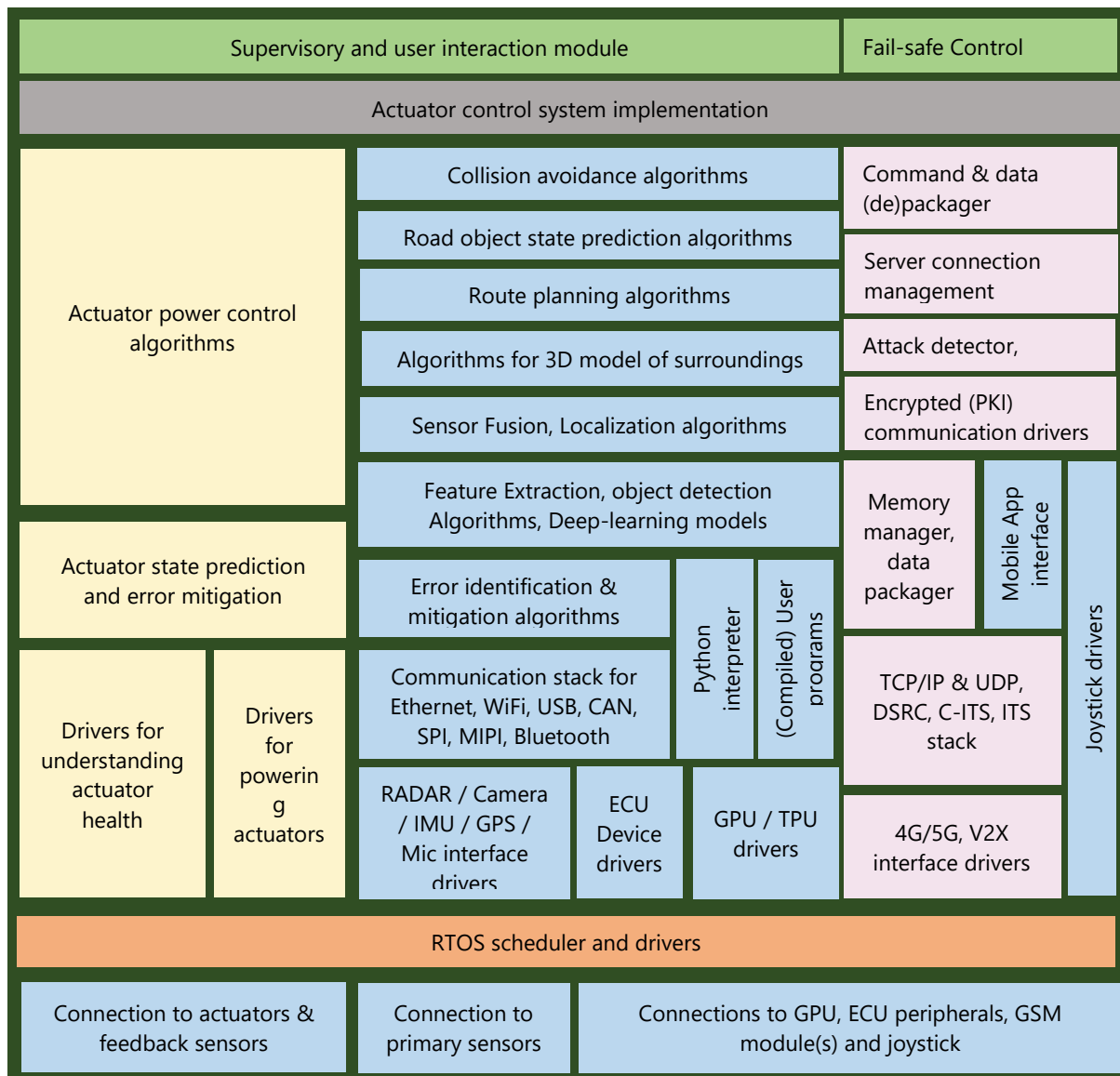
Figure 4: Software architecture of the driving robot
