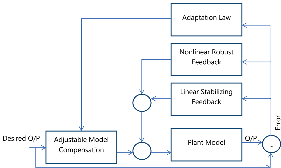
Figure 11: Block diagram of an Adaptive Robust Control System (ARC)
