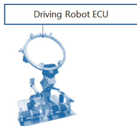
Figure 6: An implementation of mechanical actuation
