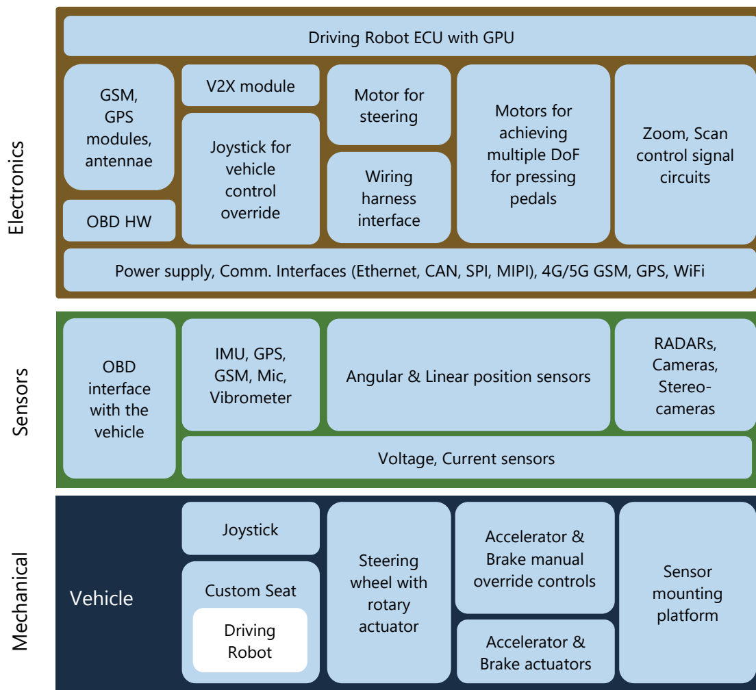
Figure 3: Architecture of physical units of the driving robot
