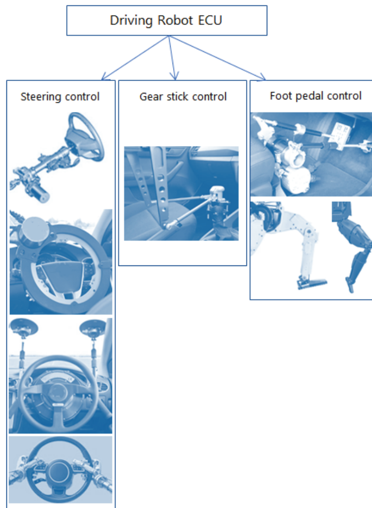
Figure 7: Mechanical actuator connection schema of the driving robot
