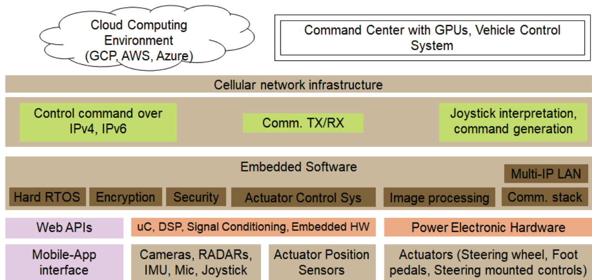
Figure 1: Architecture of the Driving Robot in the vehicle
