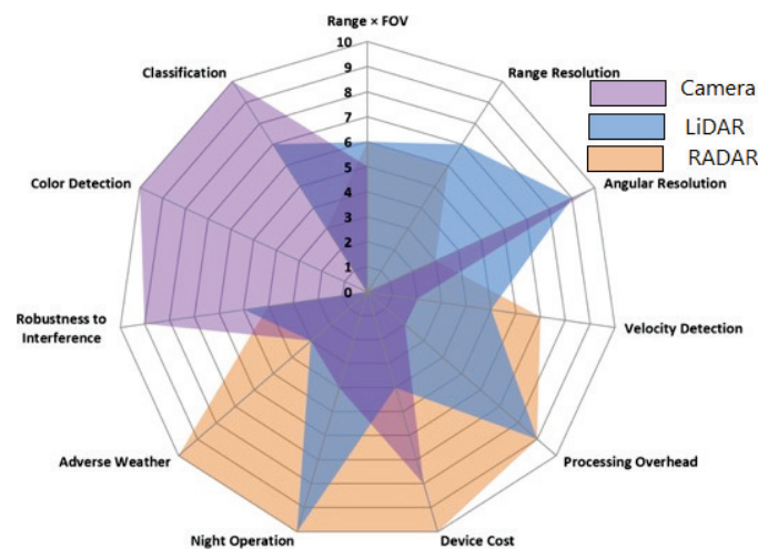
Figure 15: Comparison of the critical sensor options [55]
